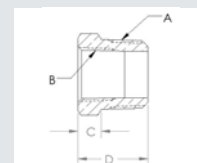
Bushing NPT to NPTFI
