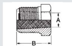
Fusible Pipe Plugs - NPTFE
