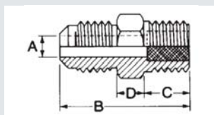
Half Union - Flare to NPTFE
