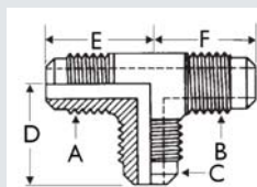
Three-Way Reducing
