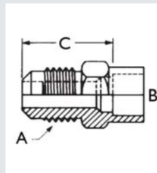
Half Union - Ext FI to Solder
