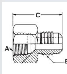
Internal FI to External FI
