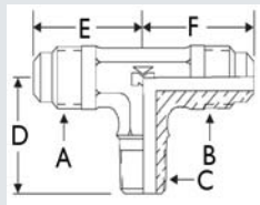
Two-Way
