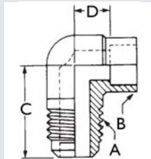
Half Union - Flare to Solder
