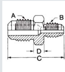
Reducing Unions - FI to FI
