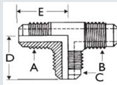
Three-Way
