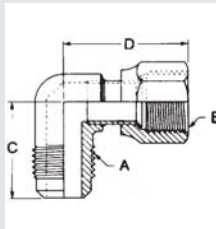
Ext FI to Int FI Swivel
