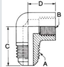
External Flare to NPTFI
