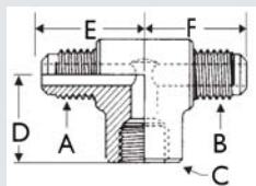
Three-Way, Internal Branch
