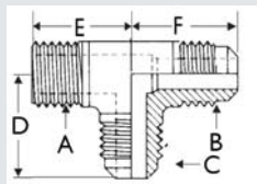
Right Angle Two-Way
